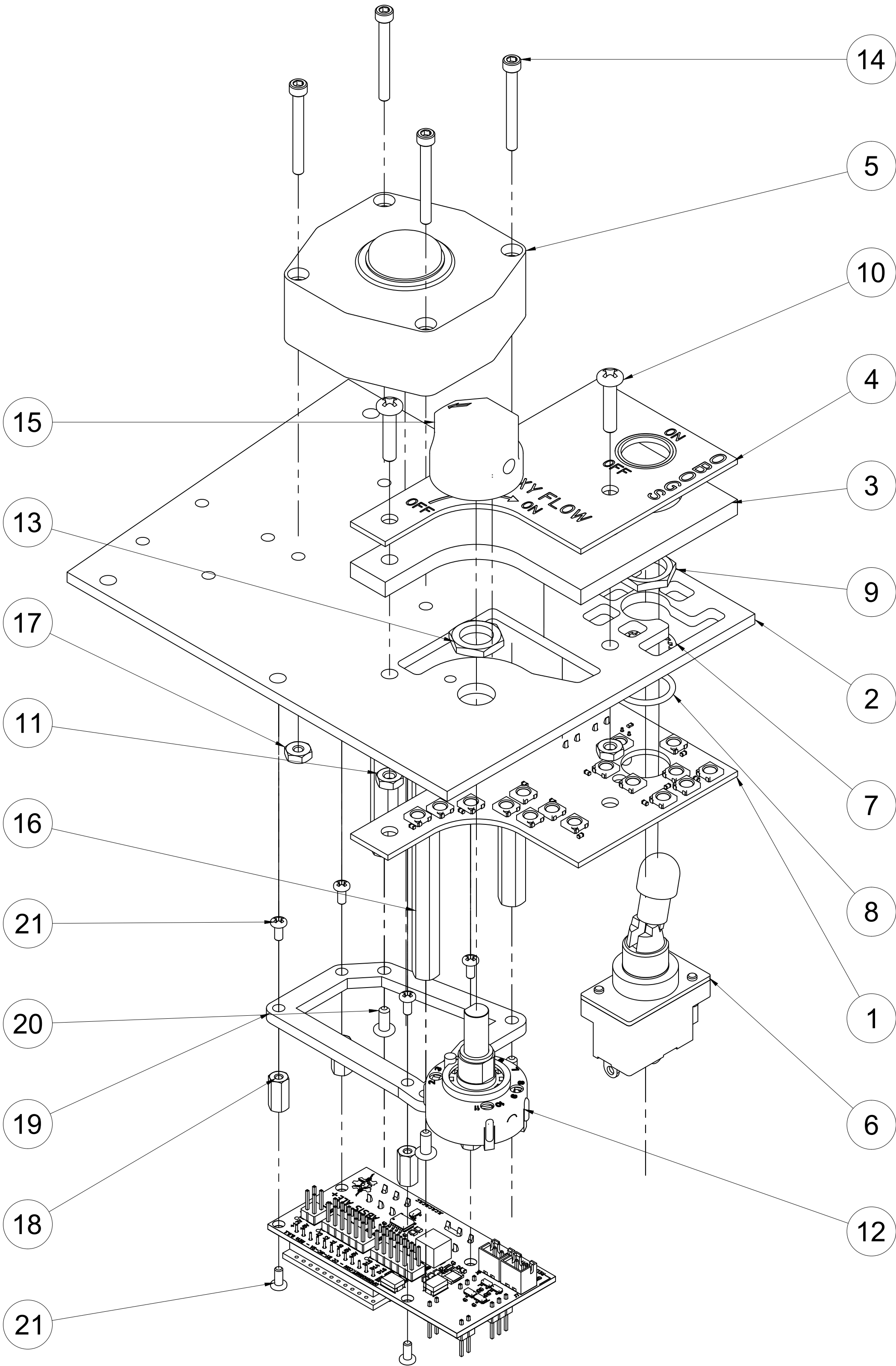
-1 ASSY SCALE 1.2:1
