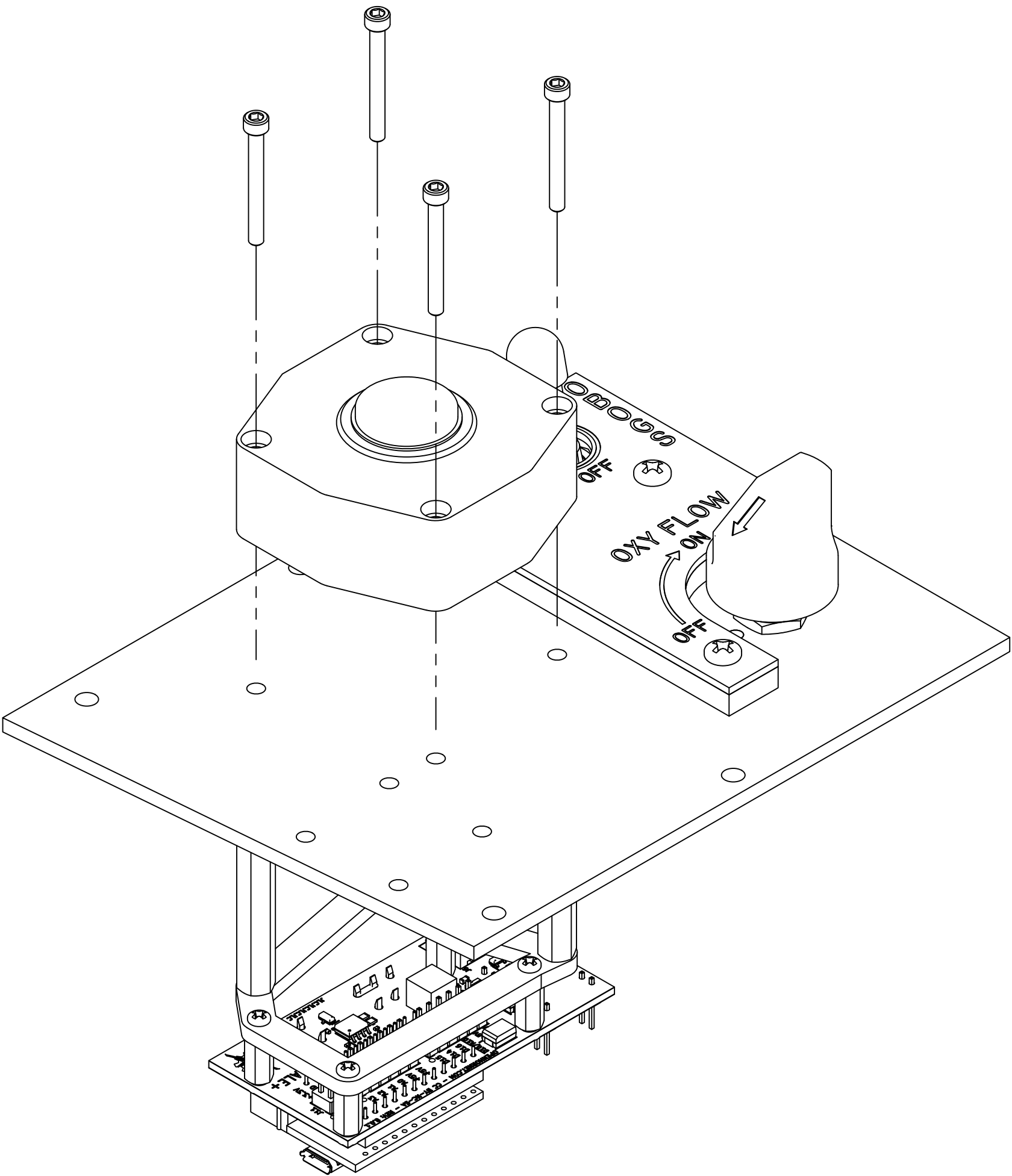
-1 ASSY SCALE 1.2:1
